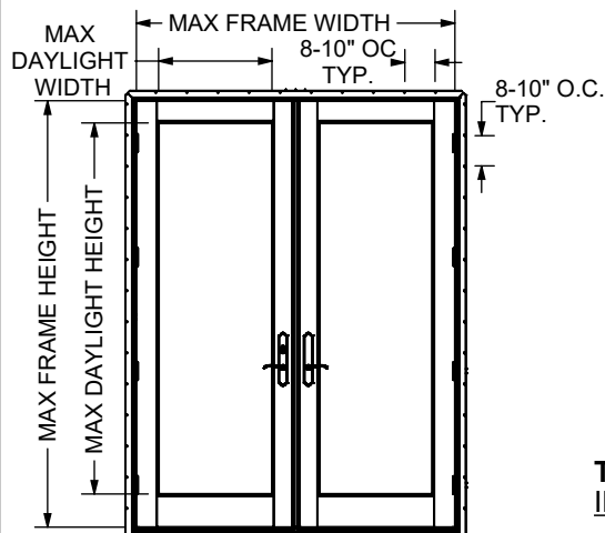
8610 Outswing French Door w/Butt Hinges Single Point Side Hinge Door Nailing Fin Installation
